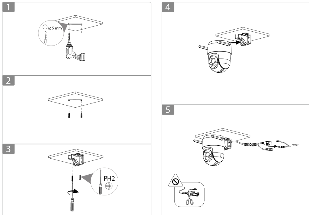
Figure 4-3 Wall mount
