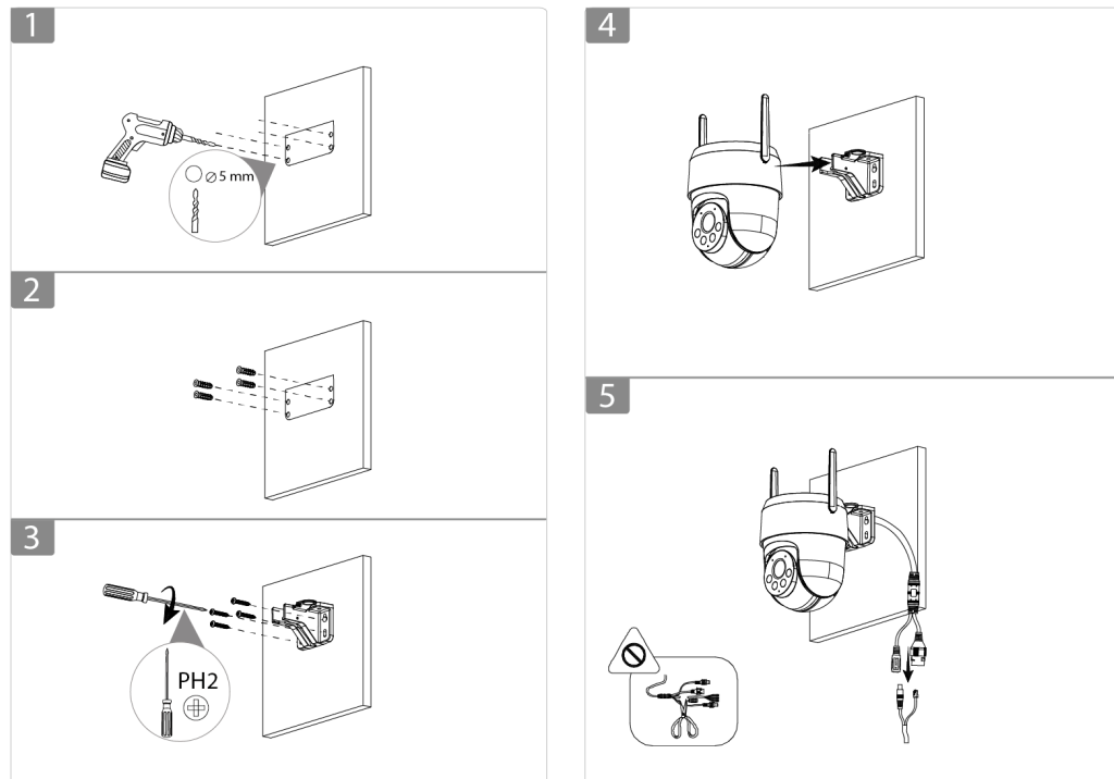
Figure 4-4 Ceiling mount
