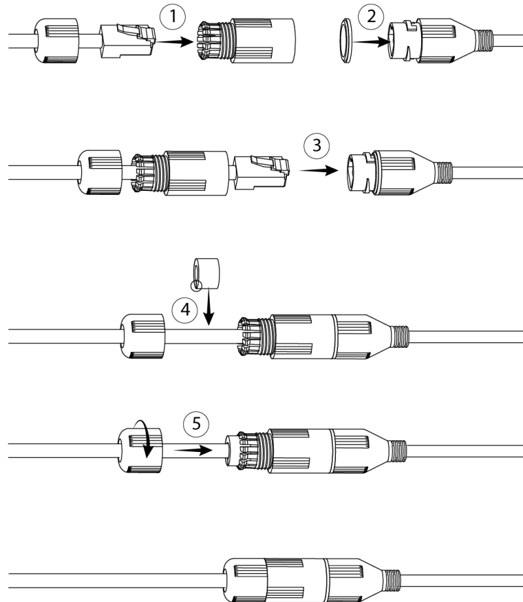
Figure 4-6 Install the waterproof connector
